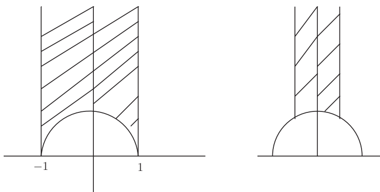
Figure 3. a) The fundamental domain of \frac{H}{\Gamma(2)} . Here H is the upper half plane, \Gamma(2) is the duality group of a sphere with four punctures; b) The fundamental domain of H/\text{SL}(2, z) .
