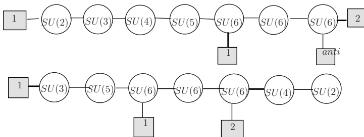
Figure 15. a) Linear quiver with weakly coupled SU ends with antisymmetric representation, b) S dual to a with SU chain of gauge groups
