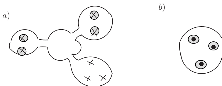
Figure 11. a) Weakly coupled description with USp ends; b) Weakly coupled description with all SUchain groups with bifundamental and fundamental matters.
