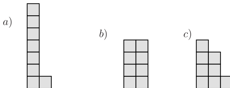
Figure 9. Young-Tableaux for a): Puncture with p_i = 1 b): Puncture with p_l = \frac{1}{2} for even l , p_l = \frac{(l-1)}{2} for odd l ; c): Puncture with p_l = \frac{l}{2} for even l , p_l = \frac{(l+1)}{2} for odd l .
