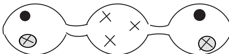
Figure 12. a) One degeneration limit of quiver gauge theory with USp ends and N - 2 SUgauge groups, here N = 4 ; b) T_N theory when we turn off the weak gauge couplings completely.
